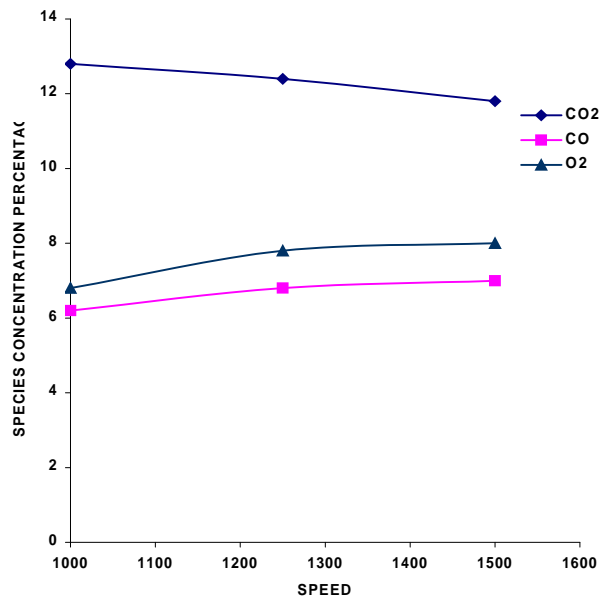
Fig (7) EFFECT OF SPEED ON SPECIES CONCENTRATION AT 80% LOAD AND 6% HYDROGEN BLENDING RATIO
