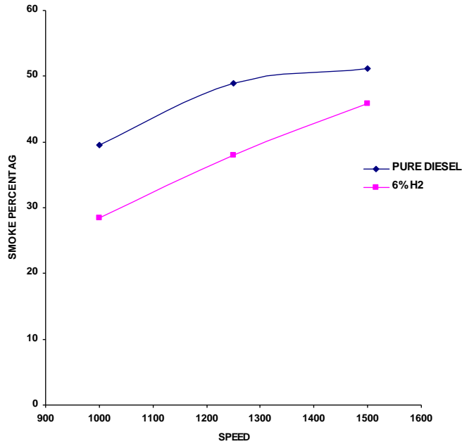
FIG (8) VARIATION OF SMOKE CONCENTRATION WITH SPEED FOR PURE DIESEL AND 6% HYDROGEN BLENDING RATIO
