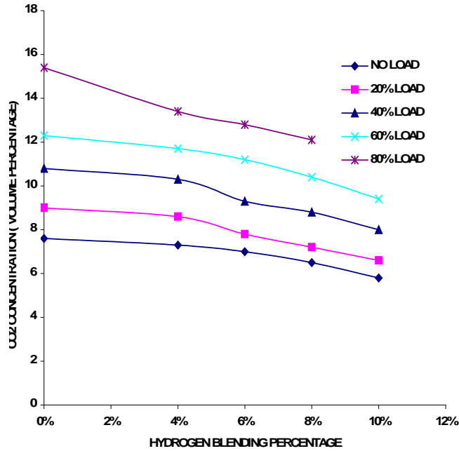
FIG (2) VARIATION OF CO 2 CONCENTRATION WITH HYDROGEN BLENDING PERCENTAGE FOR DIFFERENT LOADS AT 1000 RPM
