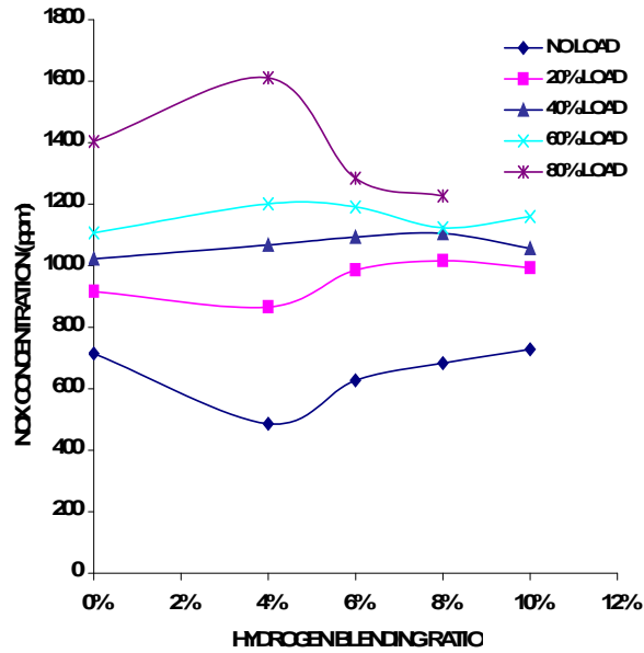
FIG(6) VARIATION OF NOX CONCENTRATION WITH HYDROGEN BLENDING RATIO FOR DIFFERENT LOADS AT 1000 RPM
