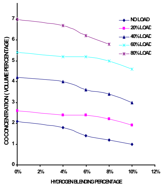
FIG (3) VARIATION OF CO CONCENTRATION WITH HYDROGEN BLENDING PERCENTAGE FOR DIFFERENT LOADS AT 1000 RPM
