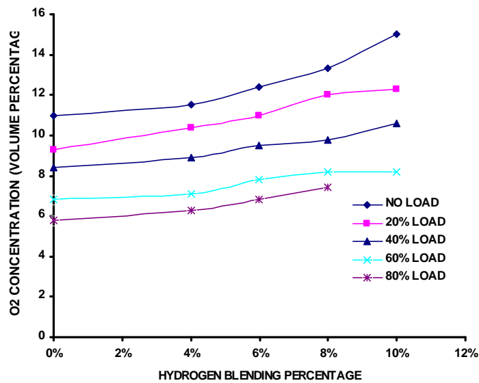
FIG (5) VARIATION OF O 2 CONCENTRATION WITH HYDROGEN BLENDING PERCENTAGE FOR DIFFERENT LOADS AT 1000 RPM
