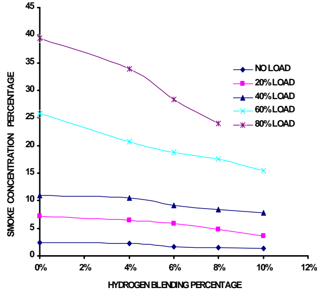
FIG (4) VARIATION OF SMOKE CONCENTRATION WITH HYDROGEN BLENDING PERCENTAGE FOR DIFFERENT LOADS AT 1000 RPM
