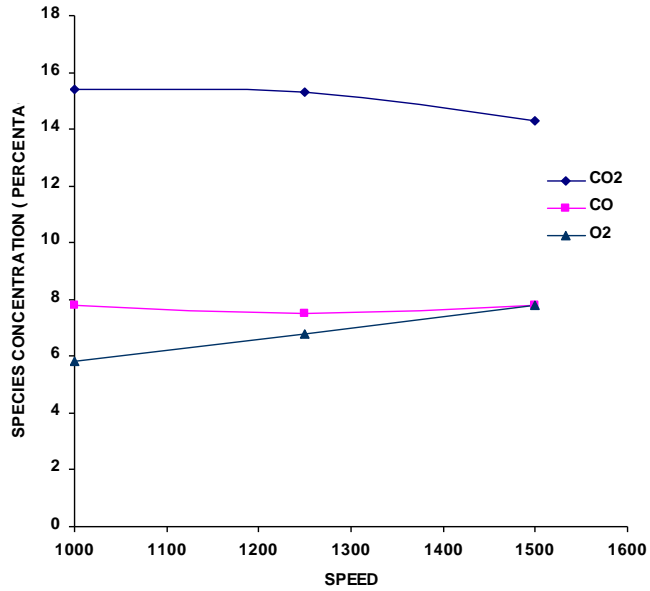
FIG (10) VARIATION OF CO 2 , CO AND O 2 CONCENTRATIONS WITH SPEED FOR PURE DIESEL AND 80% LOAD
