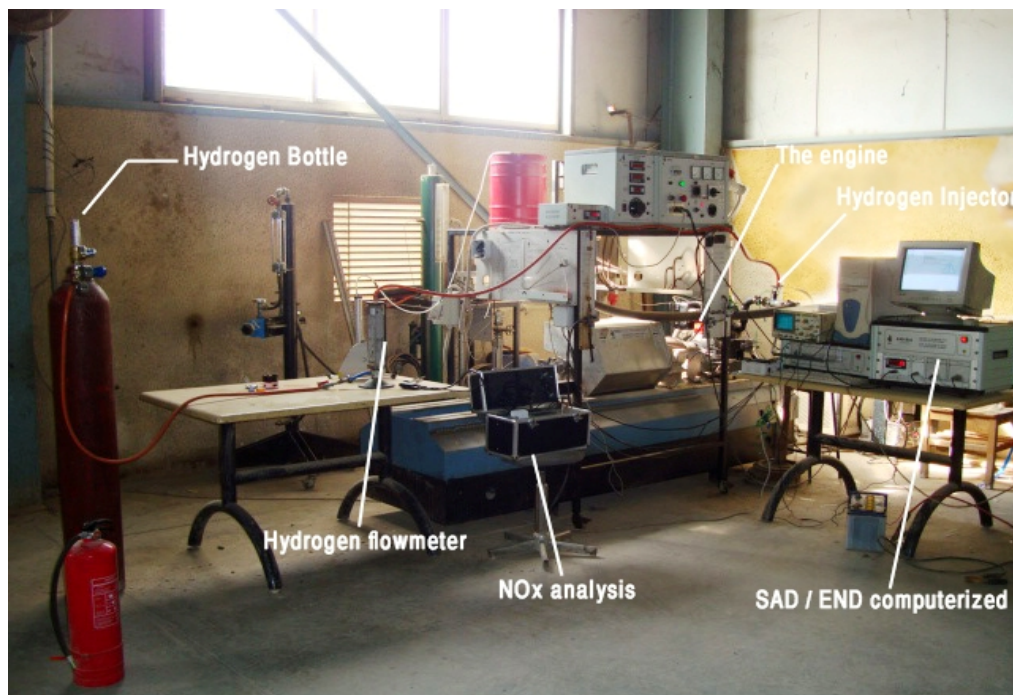
Fig (1) THE TEST RIG
