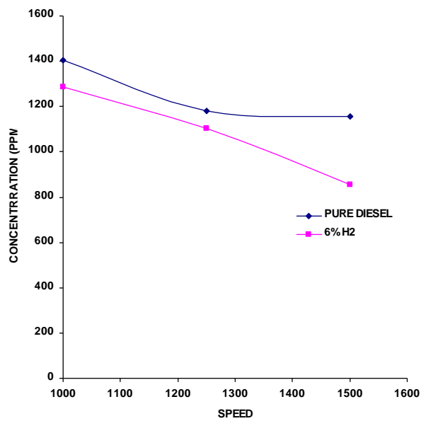
FIG (9) VARIATION OF NO x CONCENTRATION WITH SPEED FOR PURE DIESEL AND 6% HYDROGEN BLENDING RATIO
